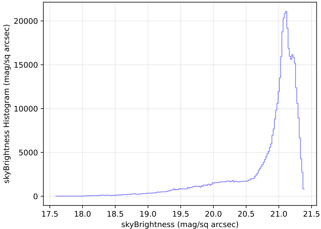
too_elab_r16_d3_giz_v3.4_10yrs All sky r band: skyBrightness Histogram
