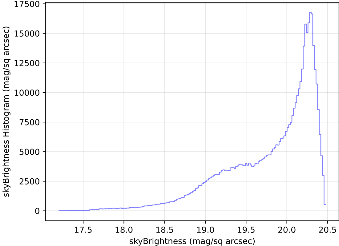
too_elab_r16_d3_giz_v3.4_10yrs All sky i band: skyBrightness Histogram
