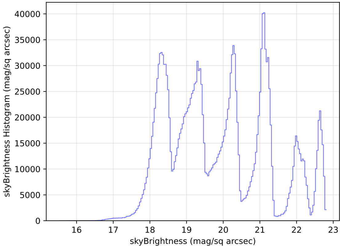
too_elab_r16_d3_giz_v3.4_10yrs All sky all bands: skyBrightness Histogram
