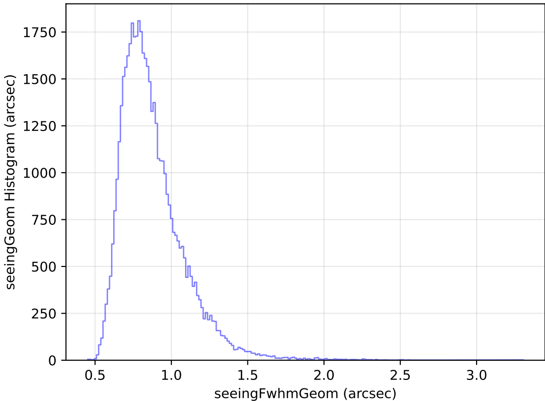
too_elab_r16_d3_giz_v3.4_10yrs Yr 1 y band: seeingGeom Histogram
