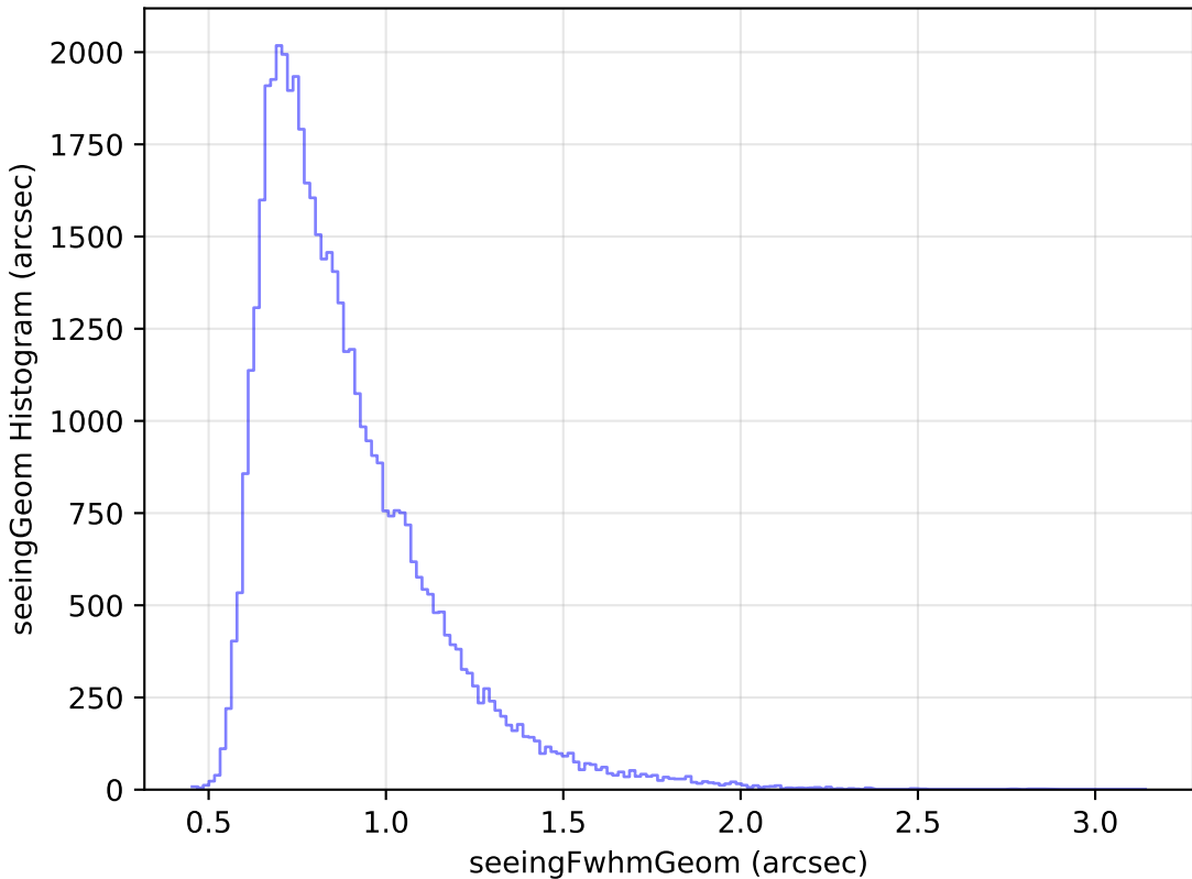
too_elab_r16_d3_giz_v3.4_10yrs Yr 1 r band: seeingGeom Histogram
