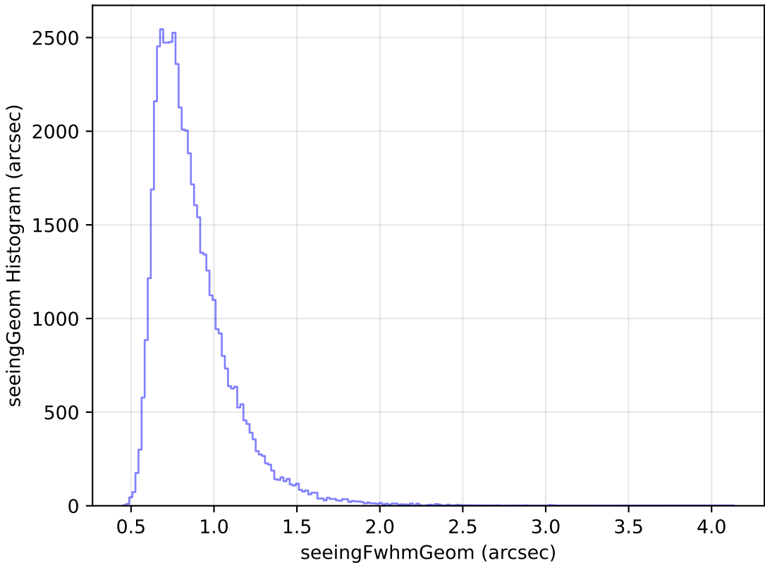
too_elab_r16_d3_giz_v3.4_10yrs Yr 1 i band: seeingGeom Histogram
