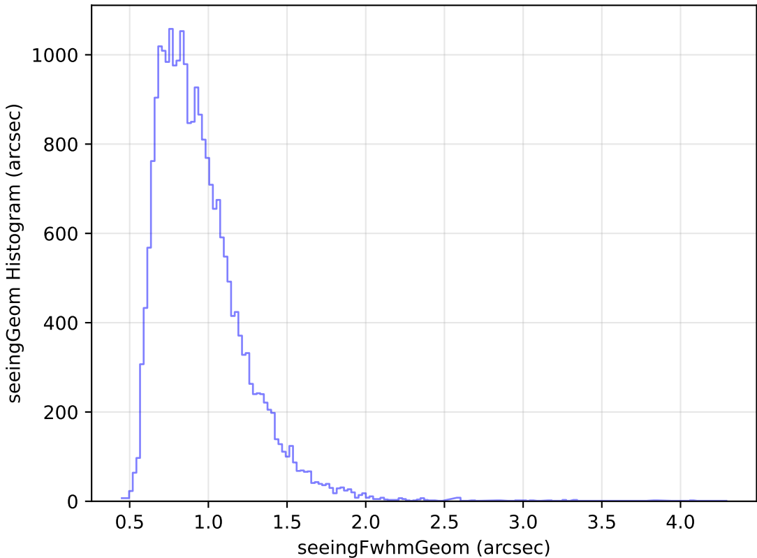
too_elab_r16_d3_giz_v3.4_10yrs Yr 1 g band: seeingGeom Histogram
