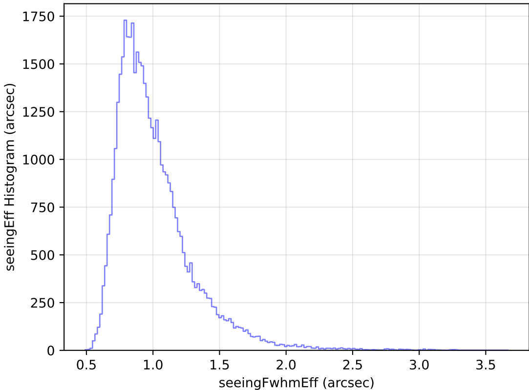
too_elab_r16_d3_giz_v3.4_10yrs Yr 1 z band: seeingEff Histogram
