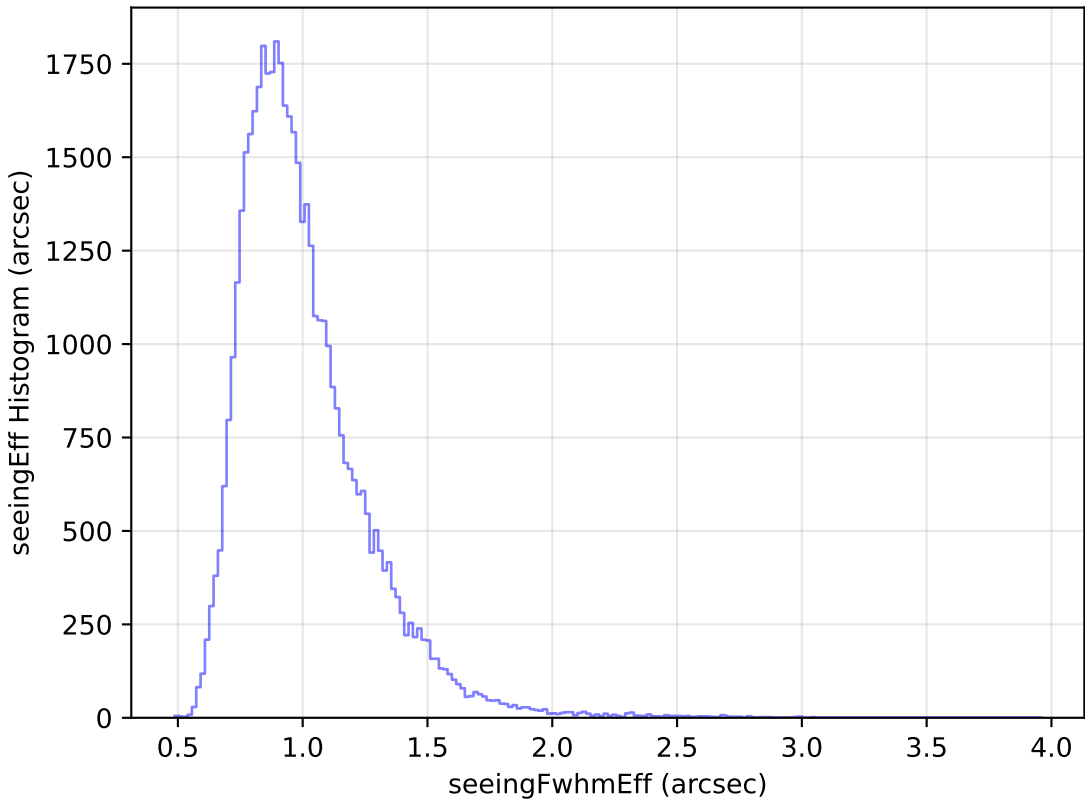
too_elab_r16_d3_giz_v3.4_10yrs Yr 1 y band: seeingEff Histogram
