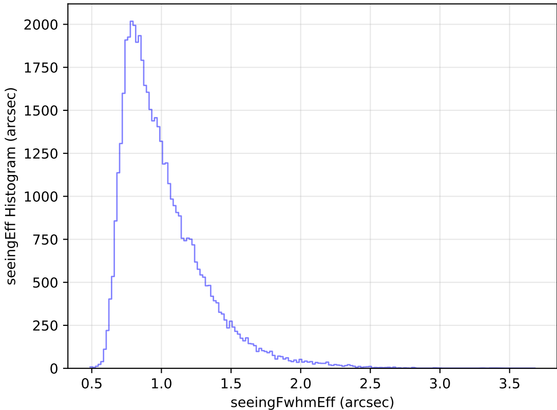
too_elab_r16_d3_giz_v3.4_10yrs Yr 1 r band: seeingEff Histogram
