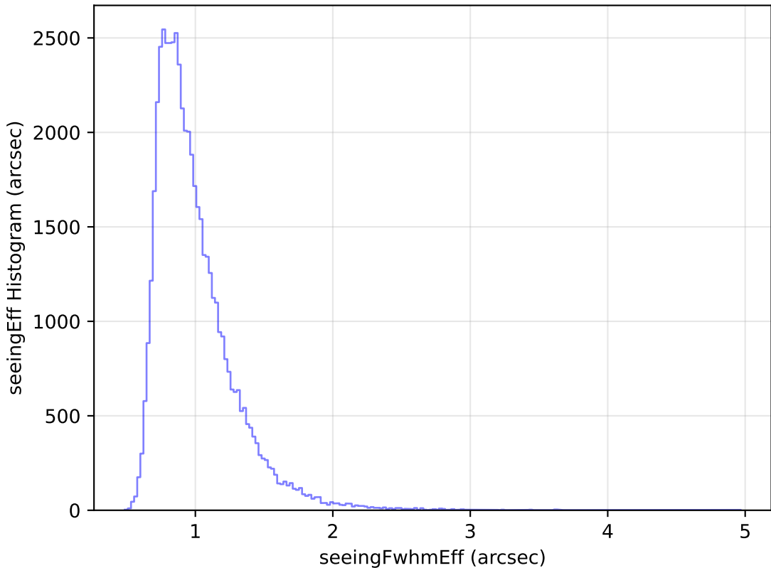
too_elab_r16_d3_giz_v3.4_10yrs Yr 1 i band: seeingEff Histogram
