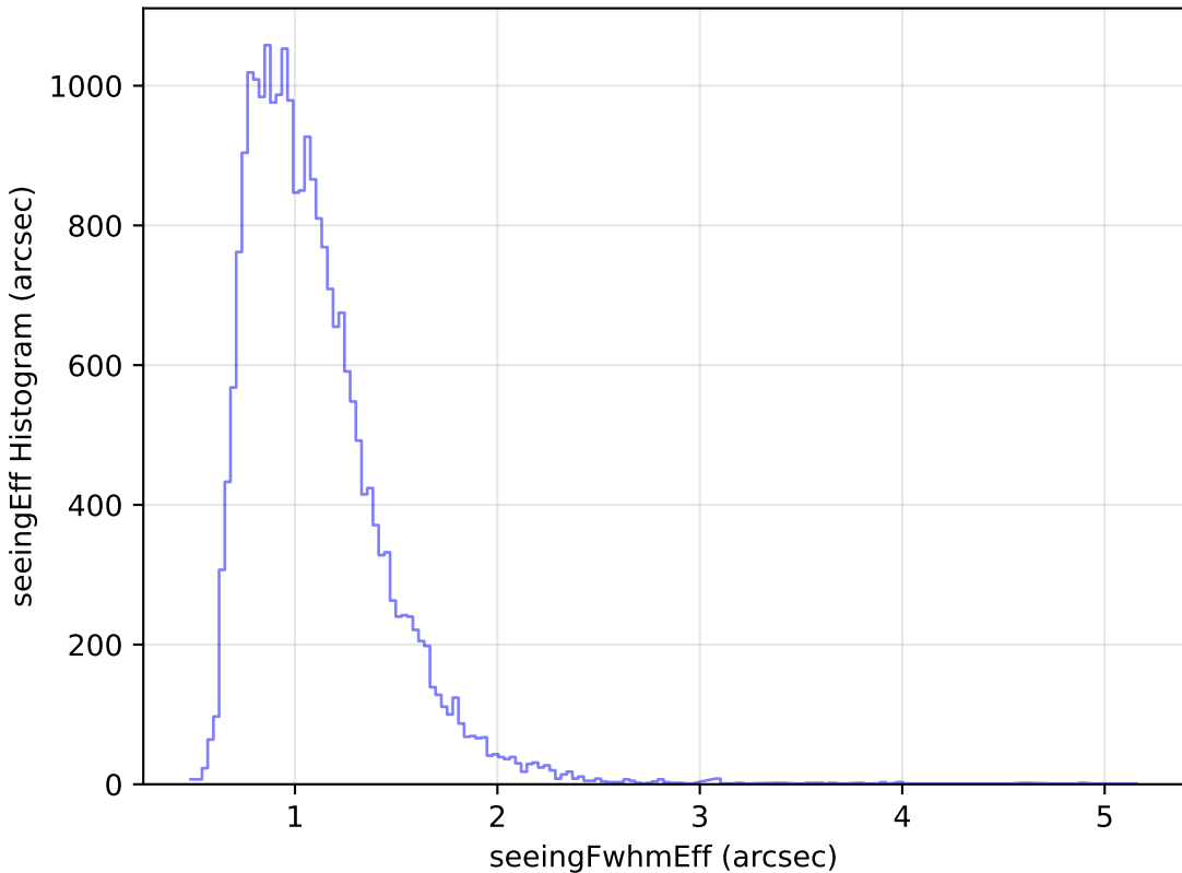
too_elab_r16_d3_giz_v3.4_10yrs Yr 1 g band: seeingEff Histogram
