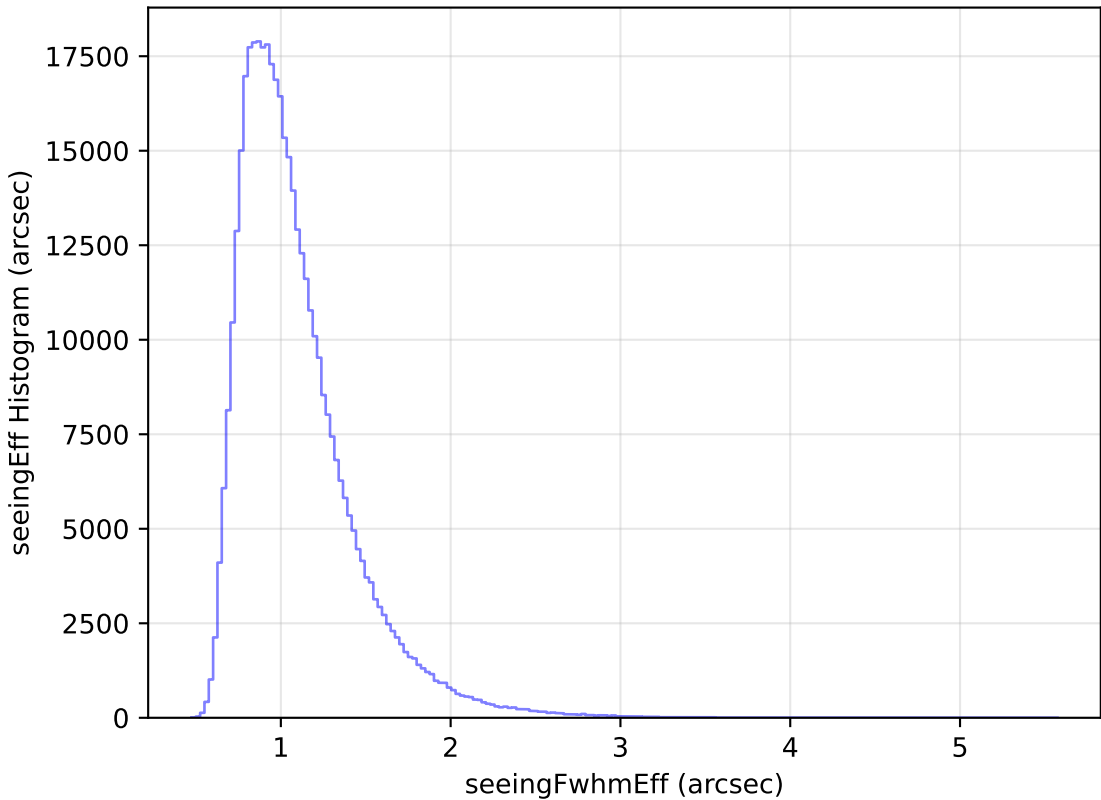
too_elab_r16_d3_giz_v3.4_10yrs WFD z band: seeingEff Histogram
