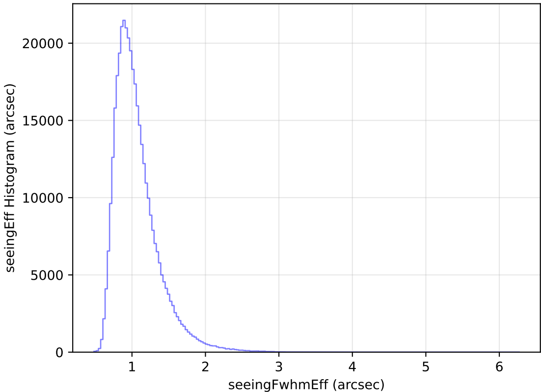
too_elab_r16_d3_giz_v3.4_10yrs WFD y band: seeingEff Histogram
