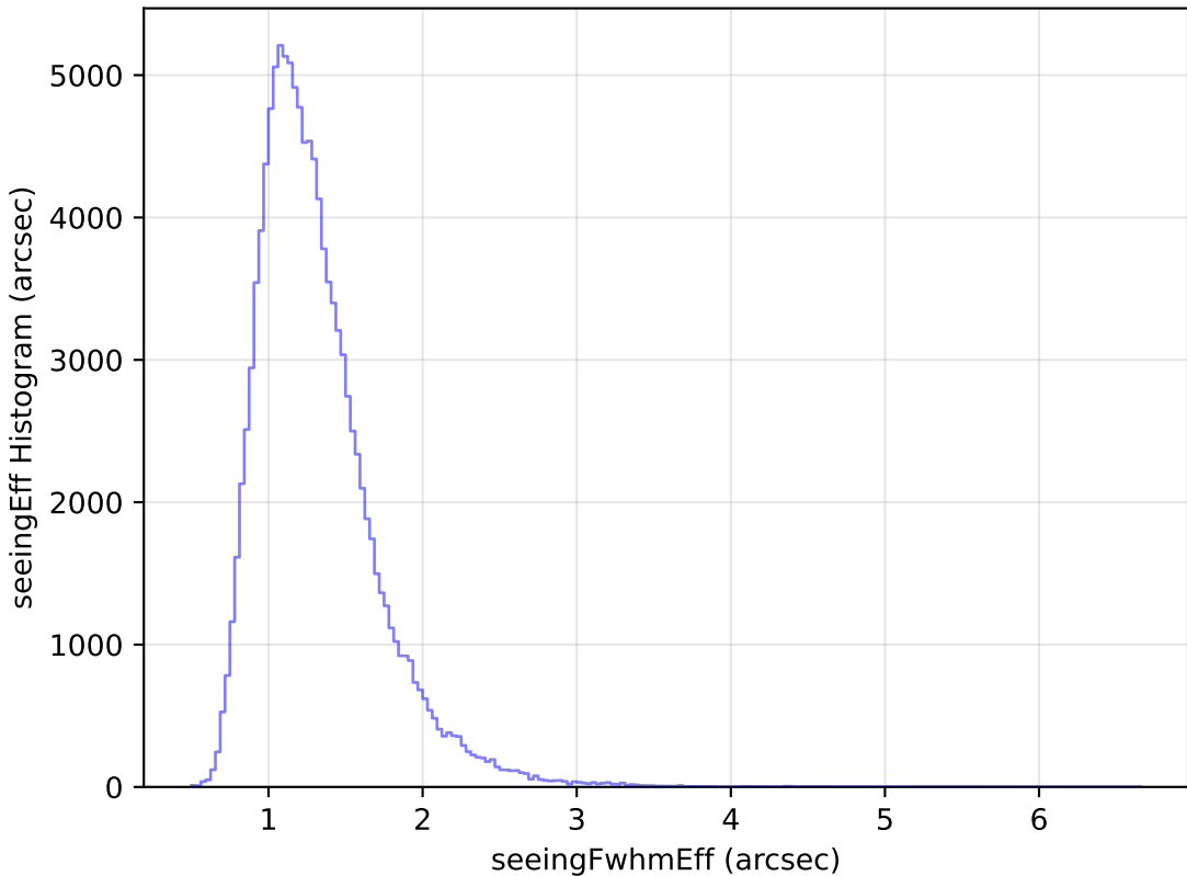
too_elab_r16_d3_giz_v3.4_10yrs WFD u band: seeingEff Histogram
