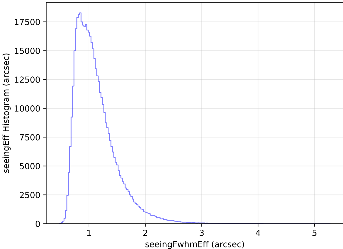
too_elab_r16_d3_giz_v3.4_10yrs WFD r band: seeingEff Histogram
