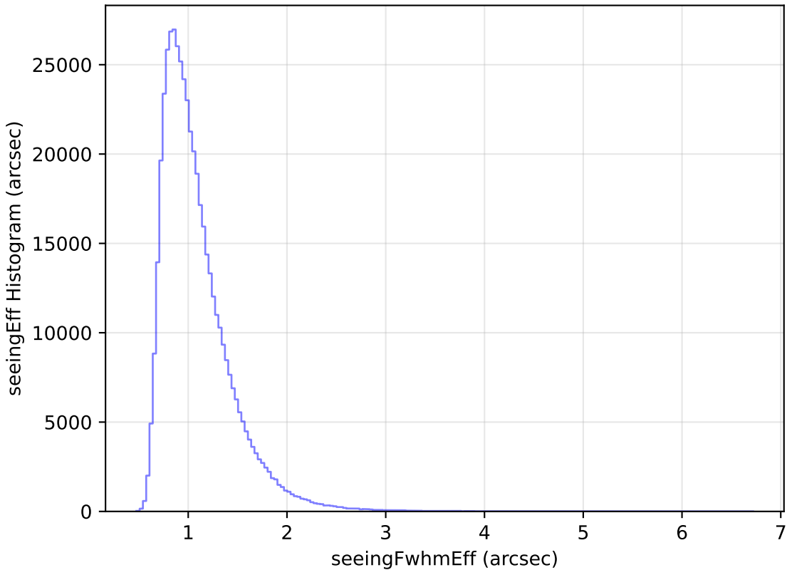
too_elab_r16_d3_giz_v3.4_10yrs WFD i band: seeingEff Histogram
