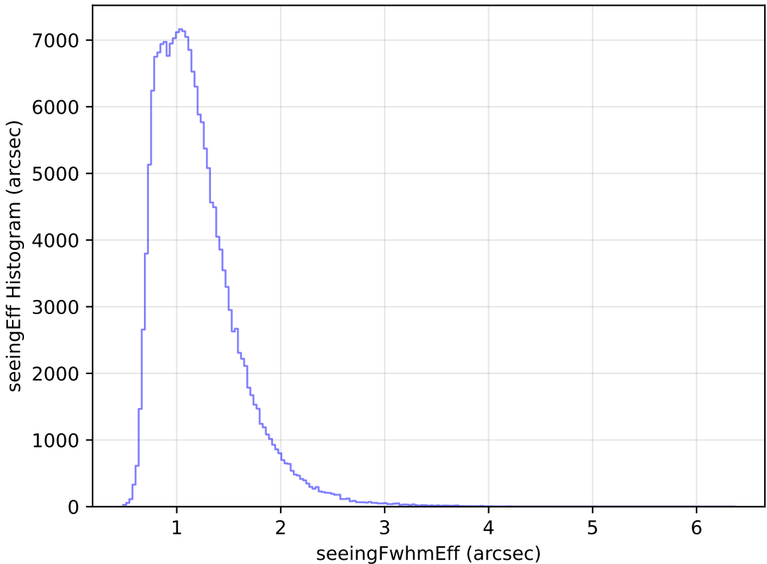
too_elab_r16_d3_giz_v3.4_10yrs WFD g band: seeingEff Histogram
