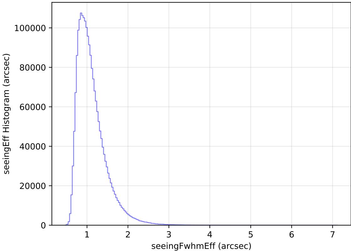
too_elab_r16_d3_giz_v3.4_10yrs WFD all bands: seeingEff Histogram
