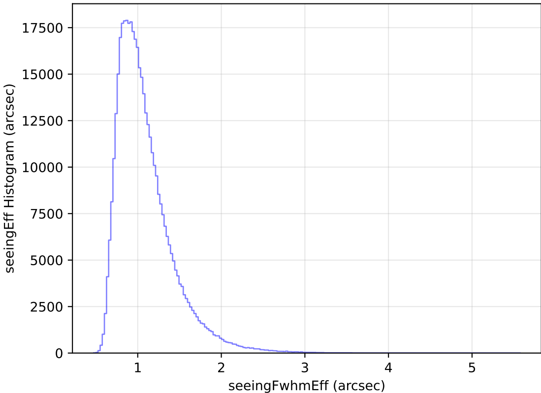
too_elab_r16_d3_giz_v3.4_10yrs All sky z band: seeingEff Histogram
