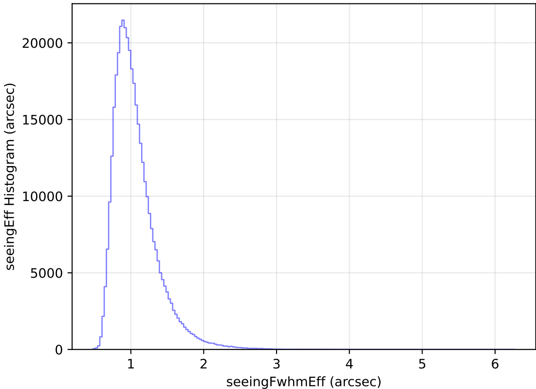
too_elab_r16_d3_giz_v3.4_10yrs All sky y band: seeingEff Histogram
