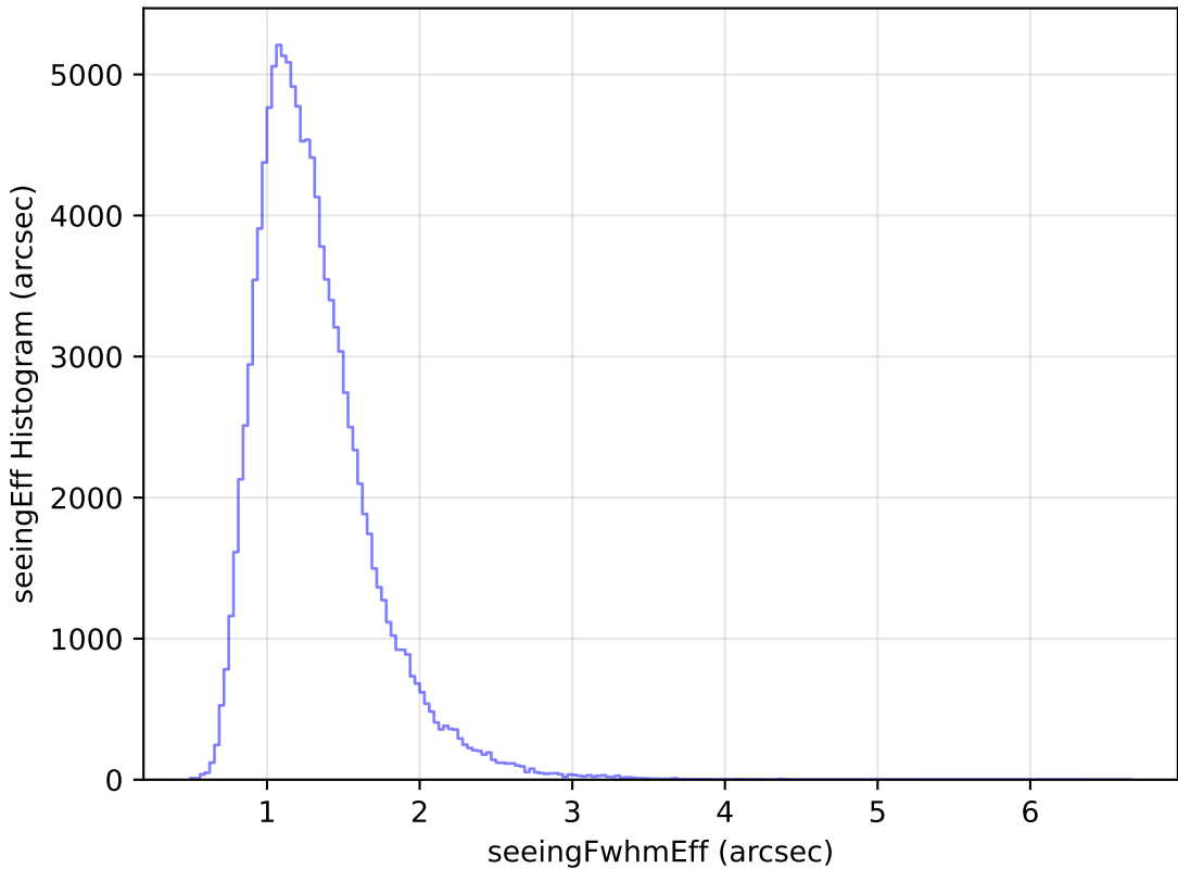
too_elab_r16_d3_giz_v3.4_10yrs All sky u band: seeingEff Histogram
