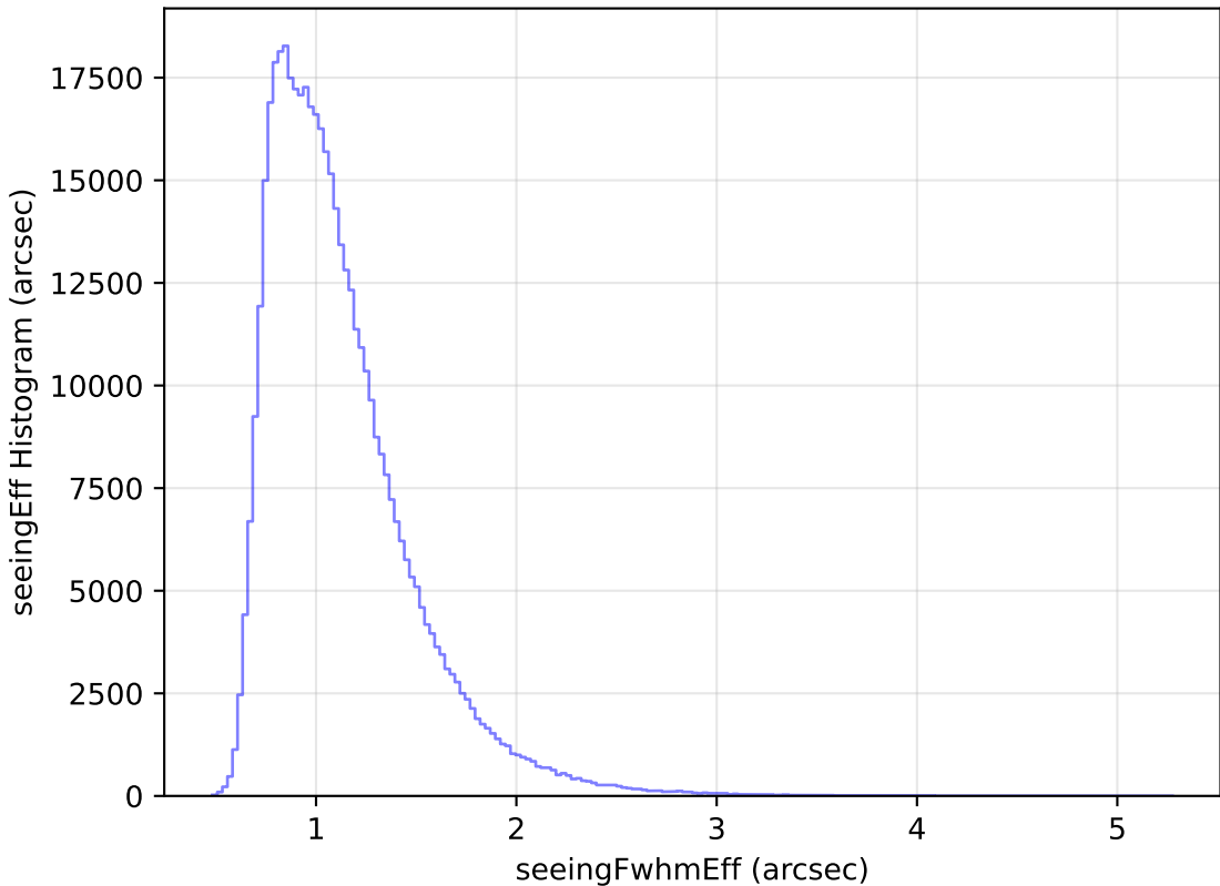
too_elab_r16_d3_giz_v3.4_10yrs All sky r band: seeingEff Histogram
