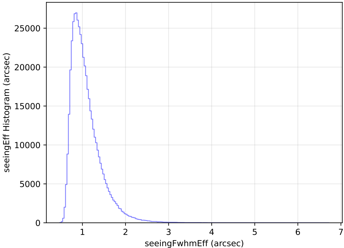
too_elab_r16_d3_giz_v3.4_10yrs All sky i band: seeingEff Histogram
