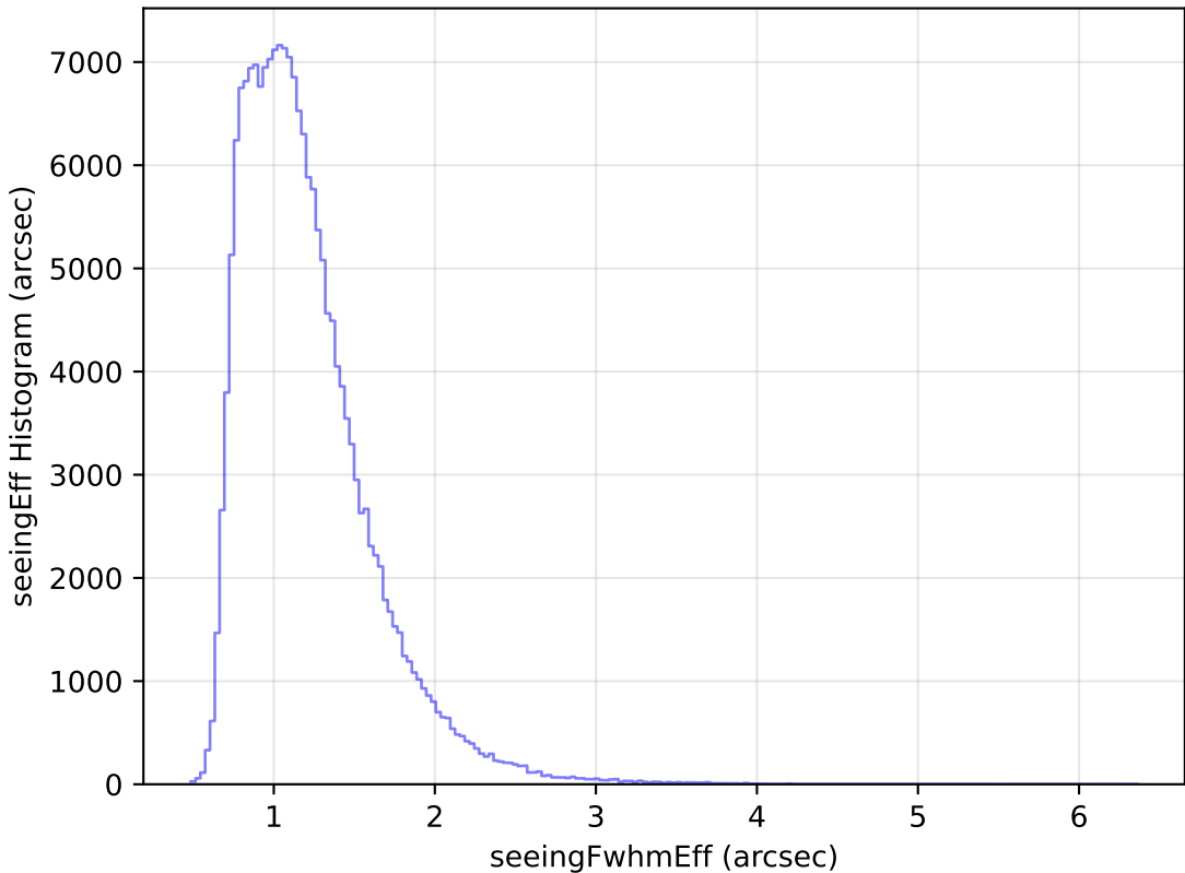
too_elab_r16_d3_giz_v3.4_10yrs All sky g band: seeingEff Histogram
