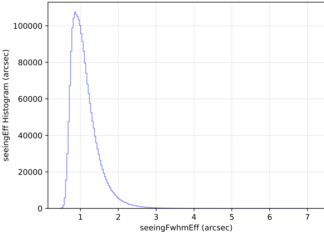
too_elab_r16_d3_giz_v3.4_10yrs All sky all bands: seeingEff Histogram
