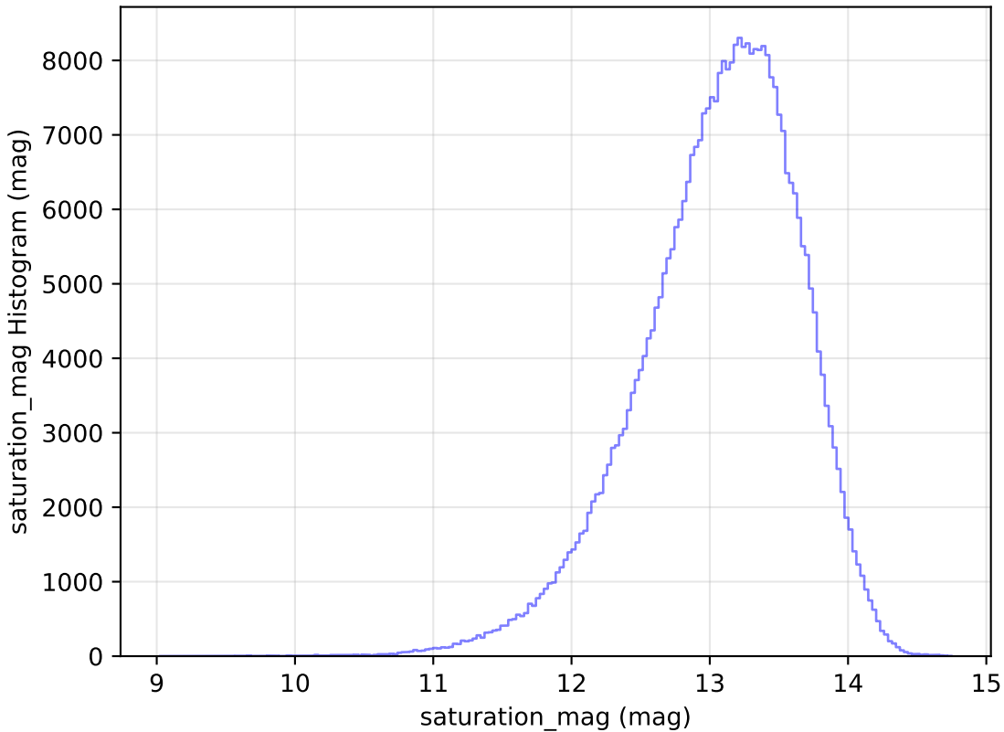
too_elab_r16_d3_giz_v3.4_10yrs WFD y band: saturation_mag Histogram
