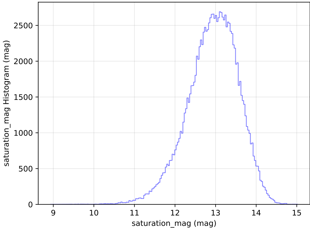
too_elab_r16_d3_giz_v3.4_10yrs WFD u band: saturation_mag Histogram
