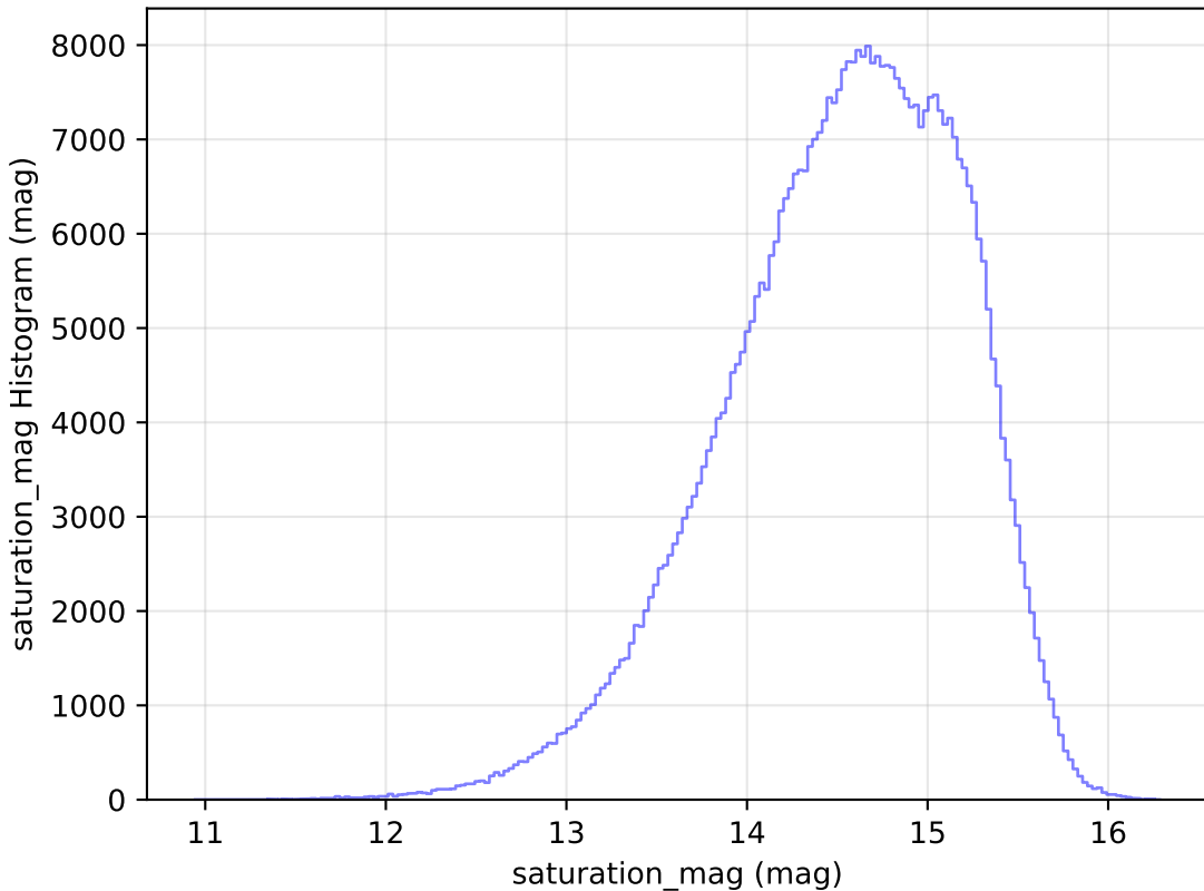
too_elab_r16_d3_giz_v3.4_10yrs WFD r band: saturation_mag Histogram
