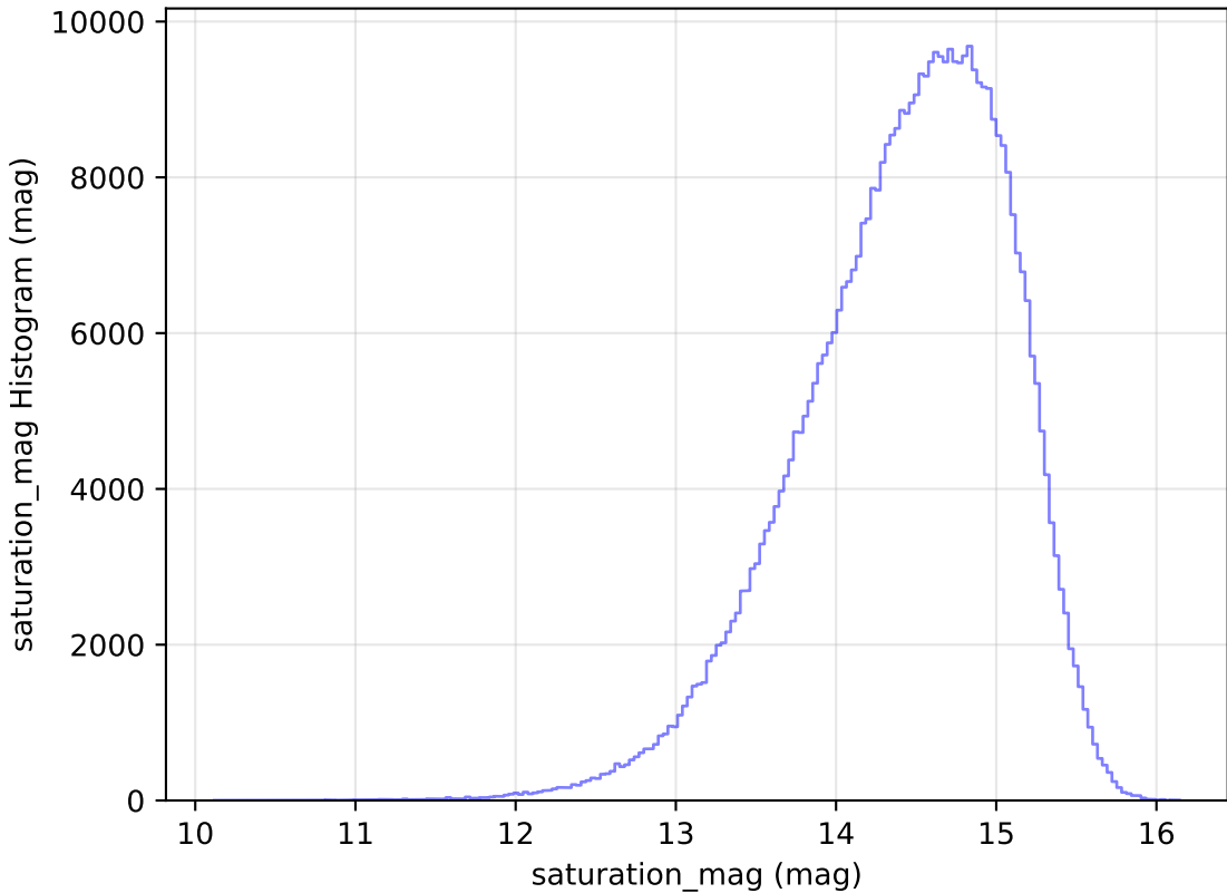
too_elab_r16_d3_giz_v3.4_10yrs WFD i band: saturation_mag Histogram
