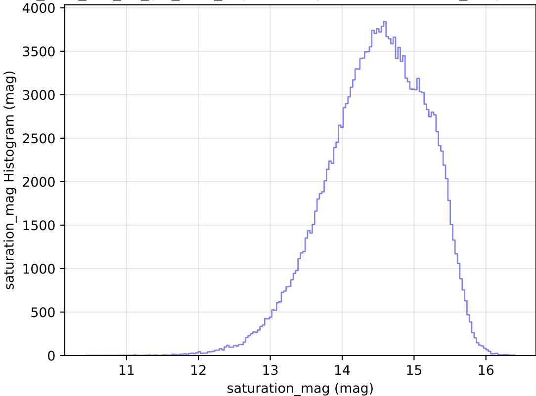
too_elab_r16_d3_giz_v3.4_10yrs WFD g band: saturation_mag Histogram
