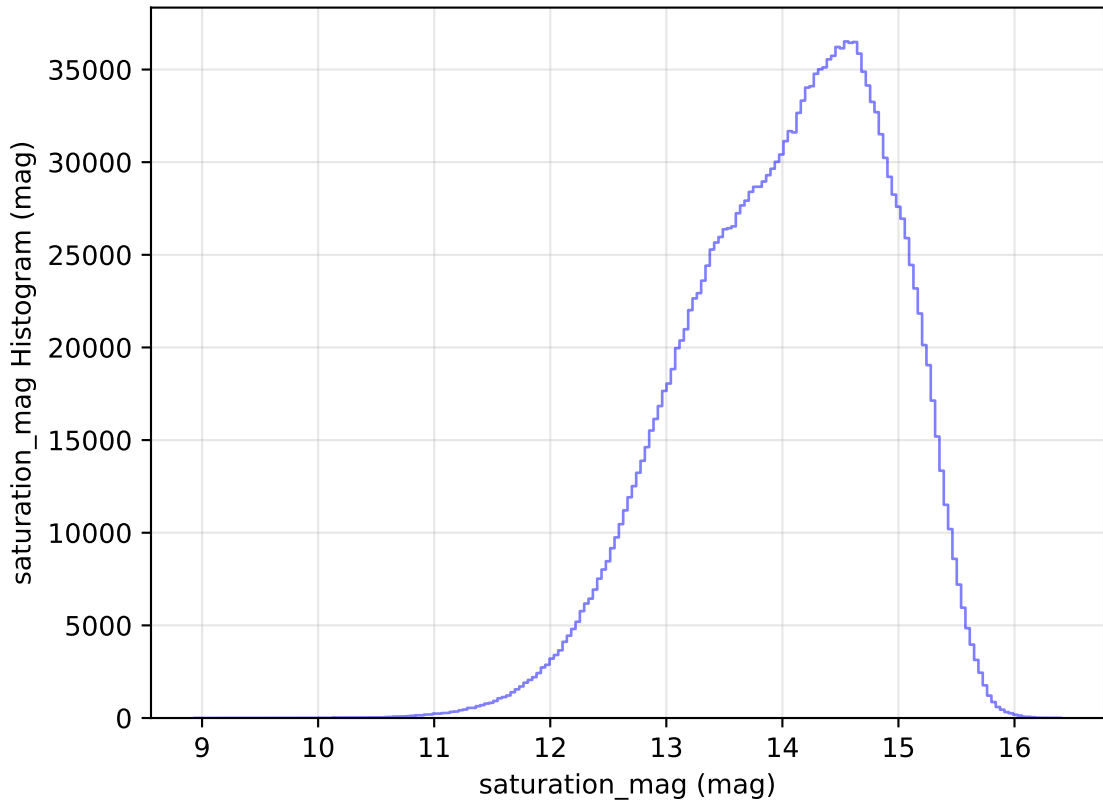
too_elab_r16_d3_giz_v3.4_10yrs WFD all bands: saturation_mag Histogram
