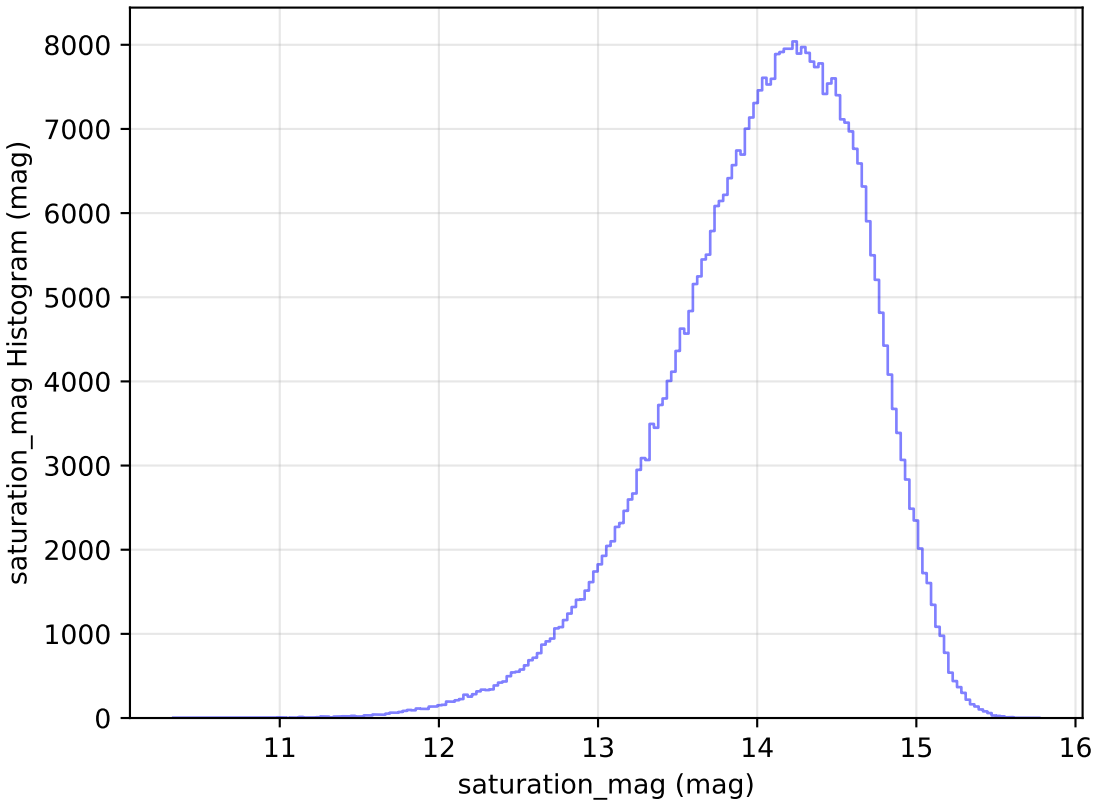
too_elab_r16_d3_giz_v3.4_10yrs All sky z band: saturation_mag Histogram
