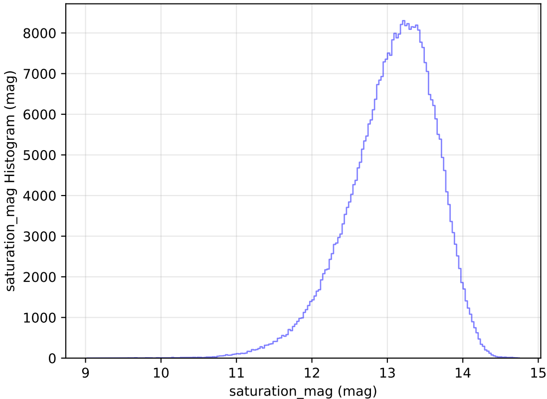
too_elab_r16_d3_giz_v3.4_10yrs All sky y band: saturation_mag Histogram
