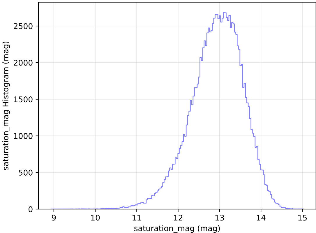
too_elab_r16_d3_giz_v3.4_10yrs All sky u band: saturation_mag Histogram
