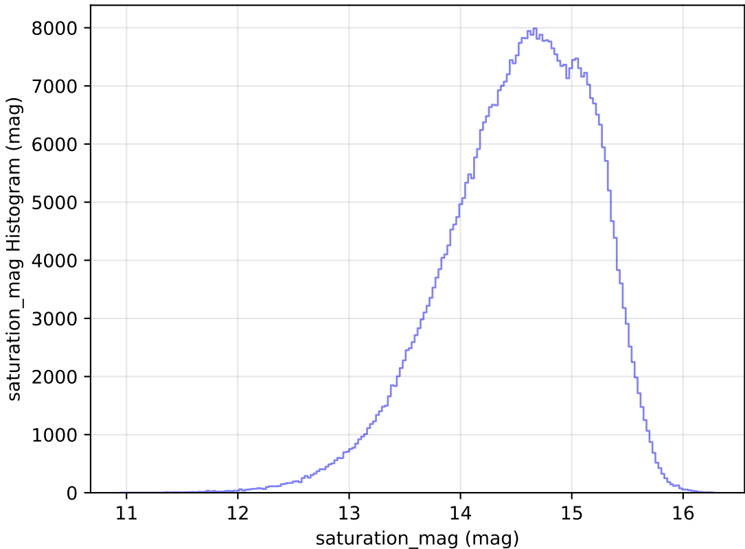
too_elab_r16_d3_giz_v3.4_10yrs All sky r band: saturation_mag Histogram
