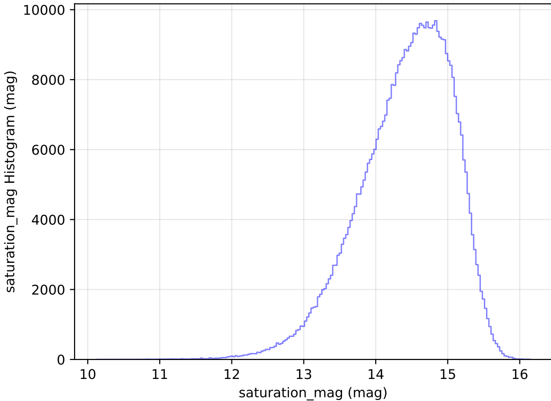
too_elab_r16_d3_giz_v3.4_10yrs All sky i band: saturation_mag Histogram
