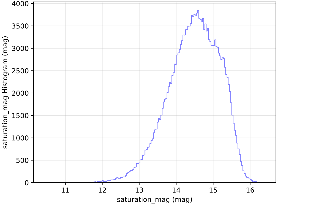
too_elab_r16_d3_giz_v3.4_10yrs All sky g band: saturation_mag Histogram
