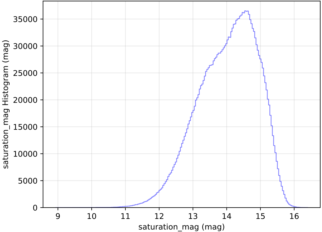
too_elab_r16_d3_giz_v3.4_10yrs All sky all bands: saturation_mag Histogram
