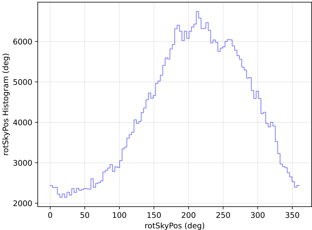
too_elab_r16_d3_giz_v3.4_10yrs WFD z band: rotSkyPos Histogram
