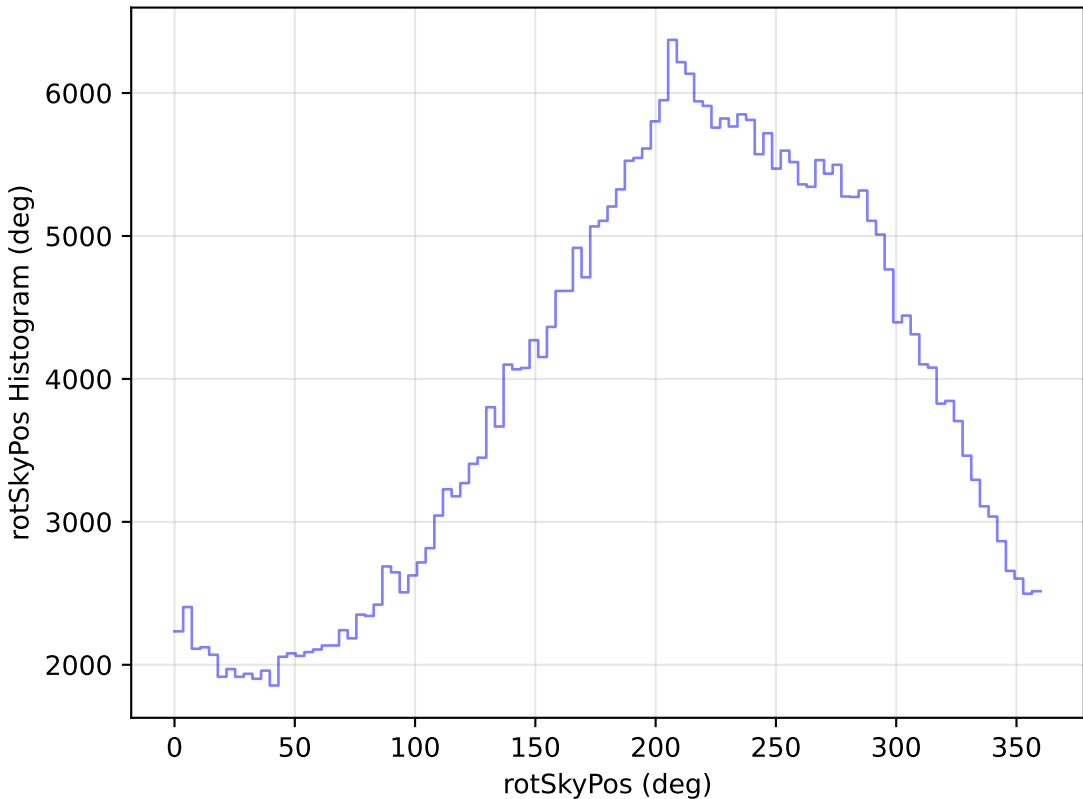
too_elab_r16_d3_giz_v3.4_10yrs WFD y band: rotSkyPos Histogram
