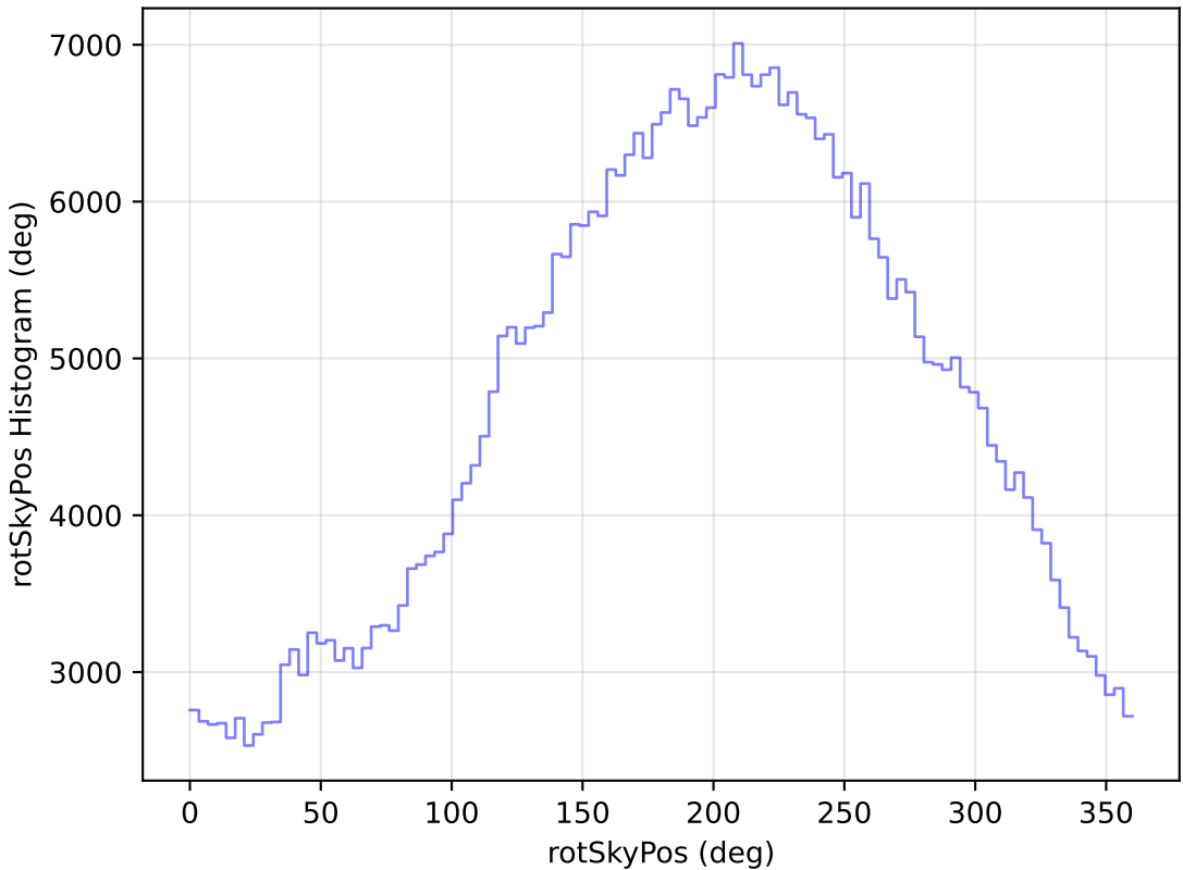
too_elab_r16_d3_giz_v3.4_10yrs WFD r band: rotSkyPos Histogram
