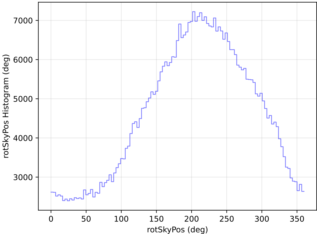
too_elab_r16_d3_giz_v3.4_10yrs WFD i band: rotSkyPos Histogram
