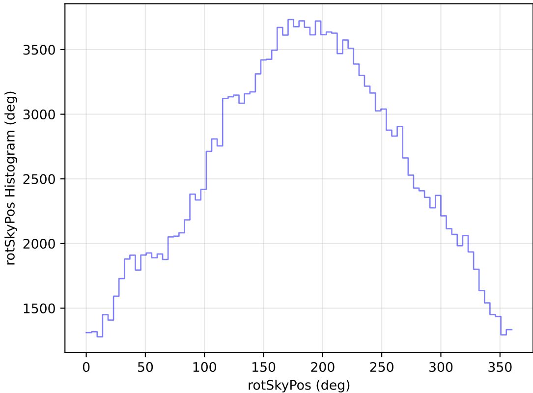
too_elab_r16_d3_giz_v3.4_10yrs WFD g band: rotSkyPos Histogram
