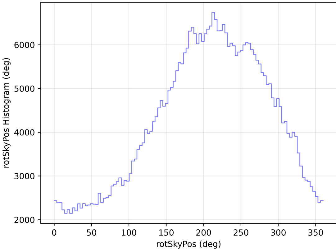
too_elab_r16_d3_giz_v3.4_10yrs All sky z band: rotSkyPos Histogram
