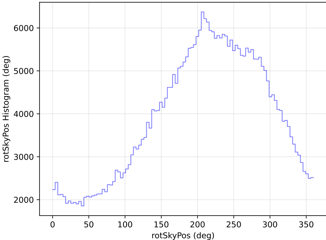
too_elab_r16_d3_giz_v3.4_10yrs All sky y band: rotSkyPos Histogram
