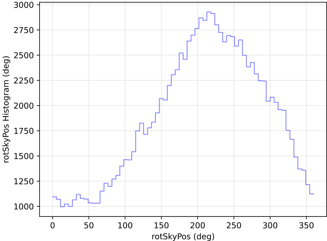
too_elab_r16_d3_giz_v3.4_10yrs All sky u band: rotSkyPos Histogram
