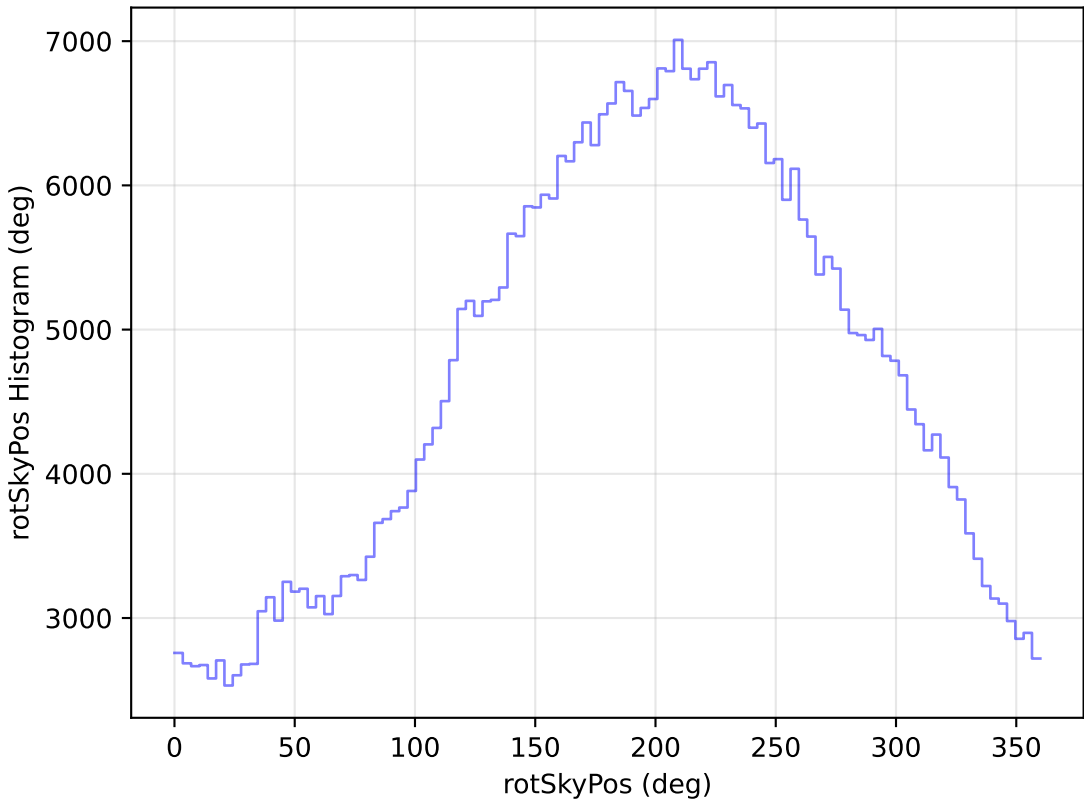
too_elab_r16_d3_giz_v3.4_10yrs All sky r band: rotSkyPos Histogram
