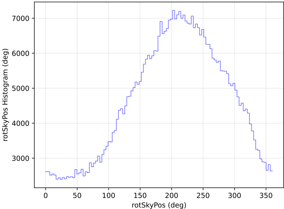
too_elab_r16_d3_giz_v3.4_10yrs All sky i band: rotSkyPos Histogram
