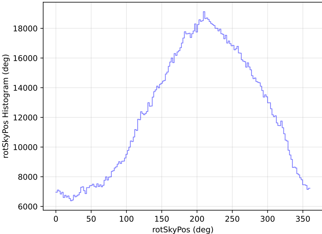
too_elab_r16_d3_giz_v3.4_10yrs All sky all bands: rotSkyPos Histogram
